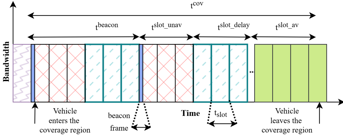
Figure 3.3: Various timing delays in a TDMA MAC Channel
